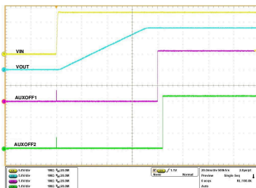
Figure 9-19. Parallel Devices Sequencing During Start-Up
