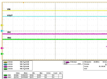
Figure 9-20. Parallel Devices Load Current During Steady State
