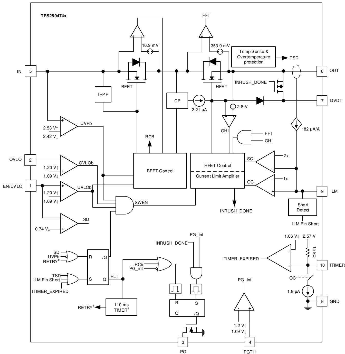
Figure 8-3. TPS25947x Block Diagram
