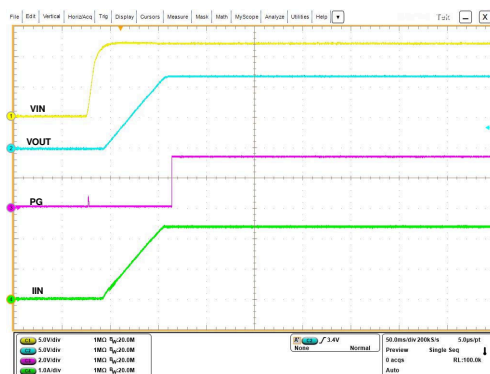
Figure 7-40. Input Hot-Plug
