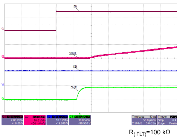
Figure 7-34. EN Turn ON Delay : EN ↑ to Output Ramp ↑
