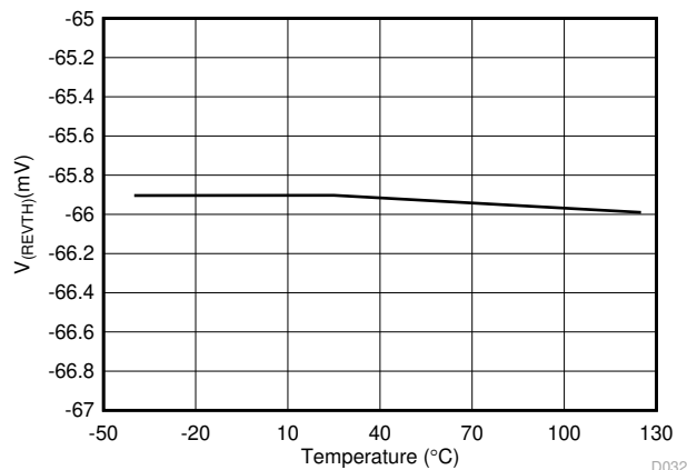
Figure 7-29. V_{(\text{REVTH})} vs Temperature
