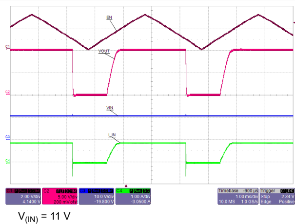
Figure 7-33. Turn ON and OFF with Enable
