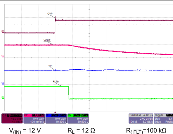
Figure 7-36. OVP Turn OFF Delay: OVP ↑ to Fault ↓
