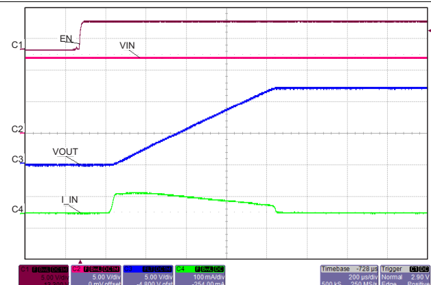
Figure 22. Transient: Output Ramp TPS25927X, C_{dVdT} = \text{OPEN} , C_{OUT} = 4.7\text{ }\mu\text{F}
