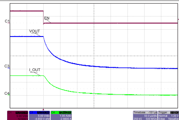
Figure 24. Transient: Turnoff Delay EN ↓
