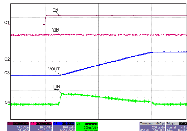
Figure 23. Transient: Output Ramp TPS25927X, V_{IN} = 18\text{ V} , C_{dVdT} = \text{OPEN} , C_{OUT} = 10\text{ }\mu\text{F}
