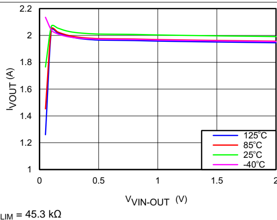
Figure 16. I_{OUT} vs V_{VIN-OUT}
