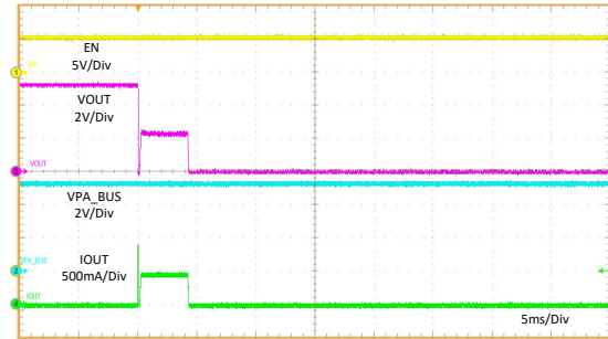
Figure 11-28. OUT short to 5.1- \Omega Load
