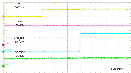
Figure 11-18. Startup Relate to EN
