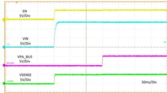
Figure 11-16. Startup Relate to VIN
