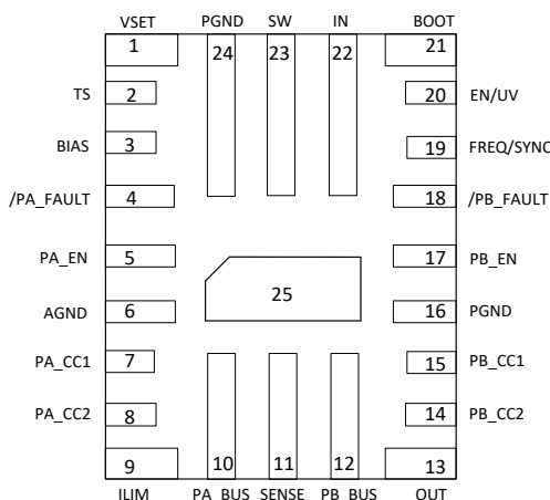
Figure 7-2. TPS25859-Q1 RPQ Package 25-Pin (QFN) Top View
