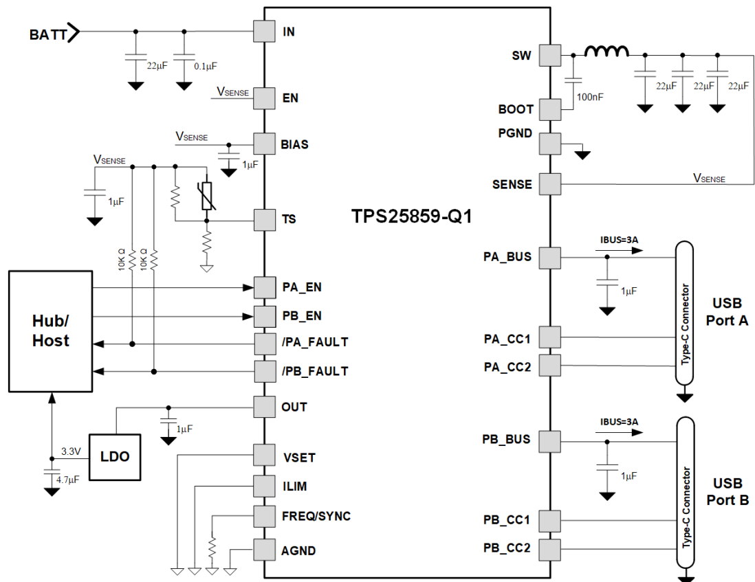
Figure 11-2. TPS25859-Q1 Typical Application Circuit for 400-kHz f_{sw}
