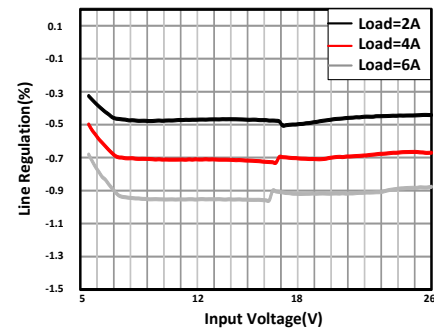
Figure 11-6. Line Regulation
