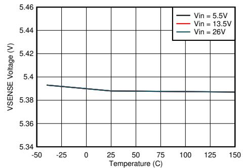
Figure 8-6. V_{SENSE} Voltage vs Junction Temperature
