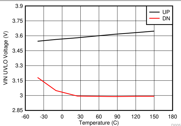
Figure 8-4. VIN UVLO Threshold
