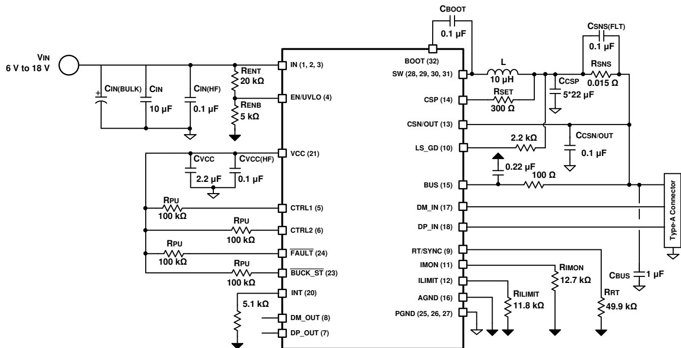
Figure 11-1. Application Circuit
