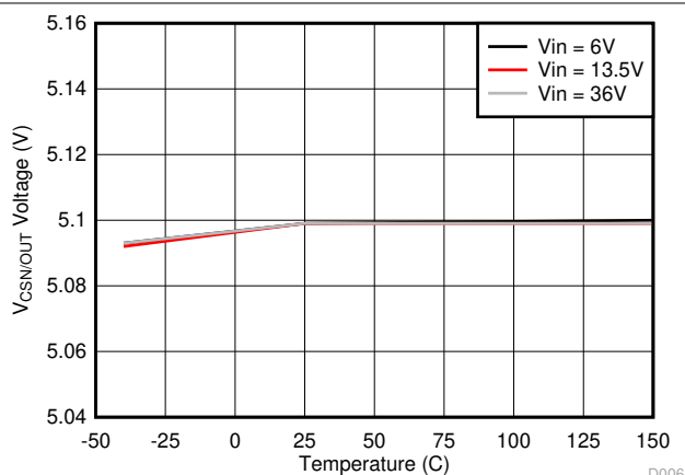
Figure 8-6. V_{CSN/OUT} Voltage vs Junction Temperature
