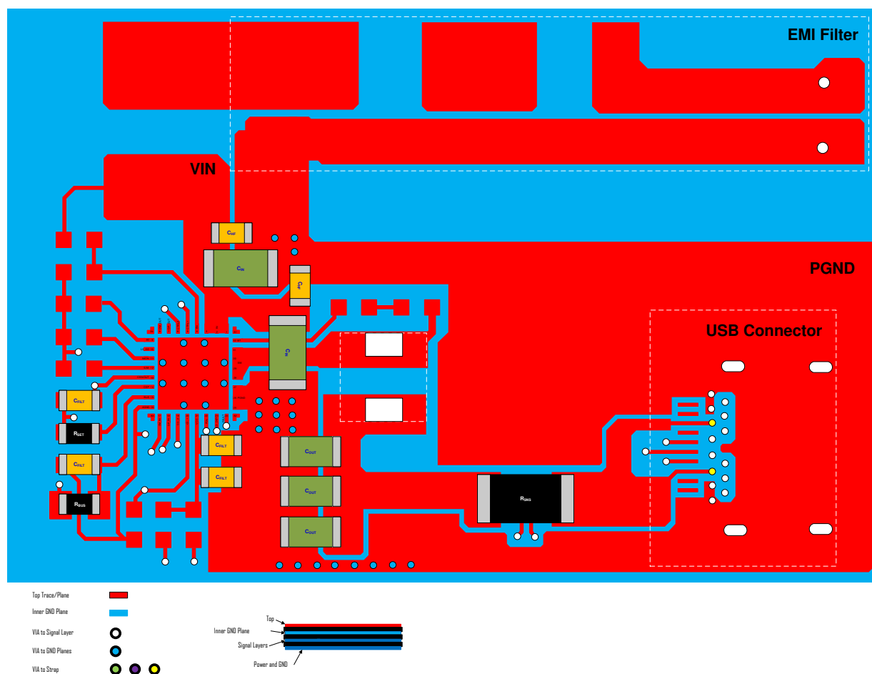
Figure 13-1. Layout
