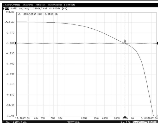
Figure 8-31. Data Transmission Characteristics vs Frequency (TPS25832-Q1)
