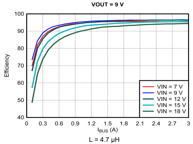
Figure 9-7. Efficiency vs Output Current ( I_{OUT} ), V OUT = 9 V
