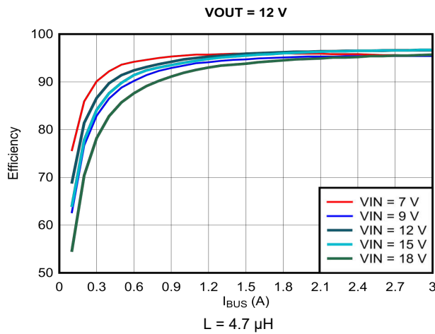
Figure 9-8. Efficiency vs Output Current ( I_{OUT} ), V OUT = 12 V
