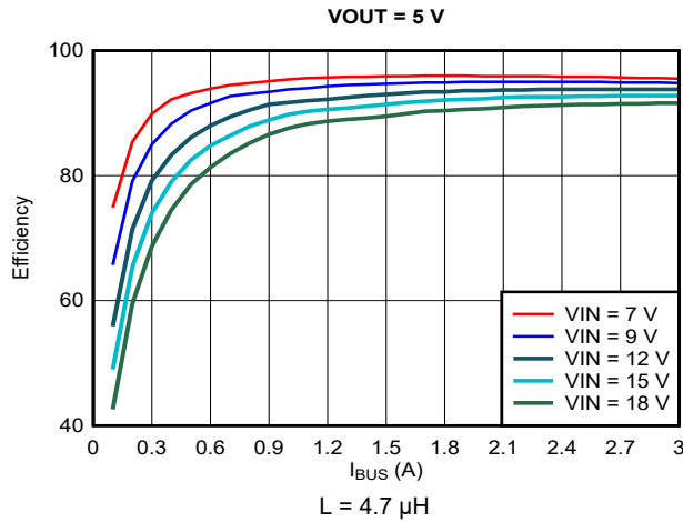
Figure 9-6. Efficiency vs Output Current ( I_{OUT} ), V OUT = 5 V
