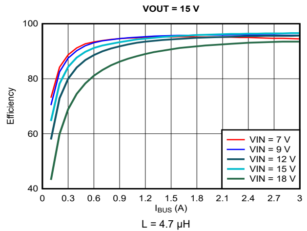
Figure 9-9. Efficiency vs Output Current ( I_{OUT} ), V OUT = 15 V
