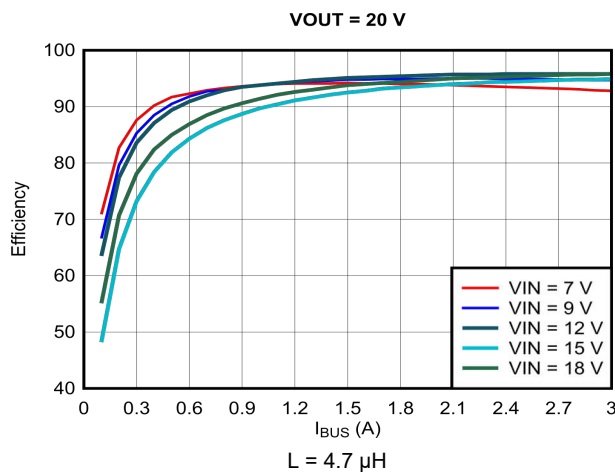
Figure 9-10. Efficiency vs Output Current ( I_{OUT} ), V OUT = 20 V
