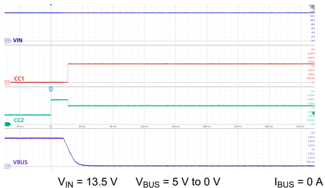
Figure 9-13. Type-C Detach
