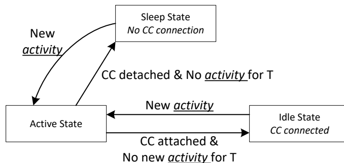
Figure 9-32. Flow Diagram for Power States
