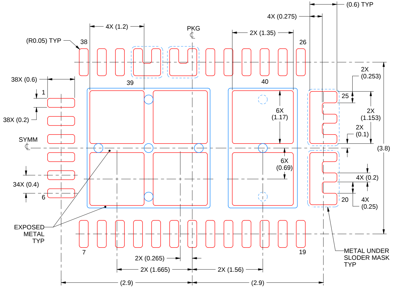
SOLDER PASTE EXAMPLE BASED ON 0.1 mm THICK STENCIL
