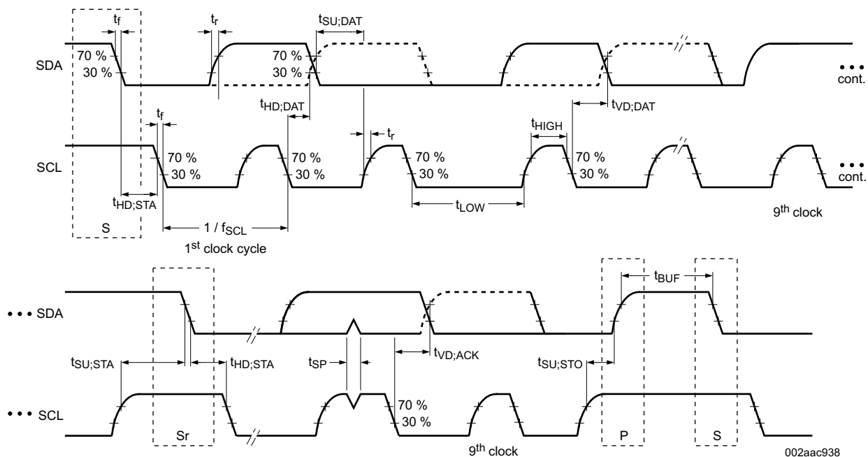
Figure 8-1. I²C Slave Interface Timing
