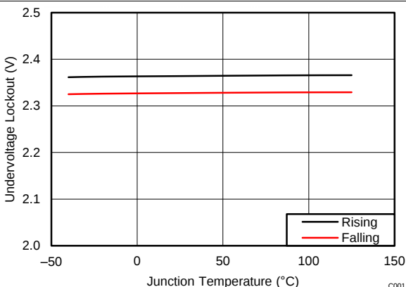
Figure 1. Under-voltage Lockout (UVLO) vs Temperature
