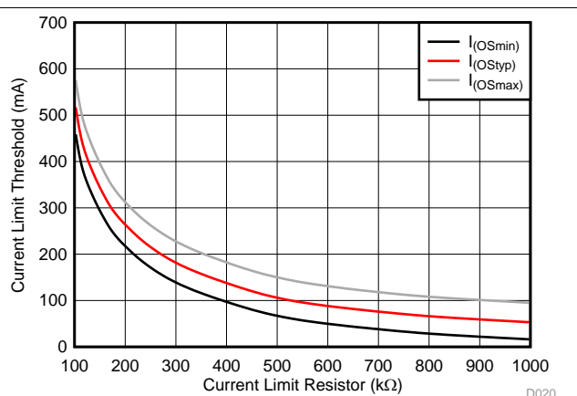
Figure 43. Current Limit Setting vs Programming Resistor II
