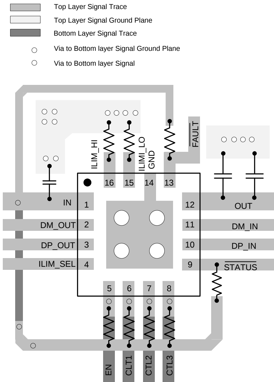
Figure 46. Layout Recommendation
