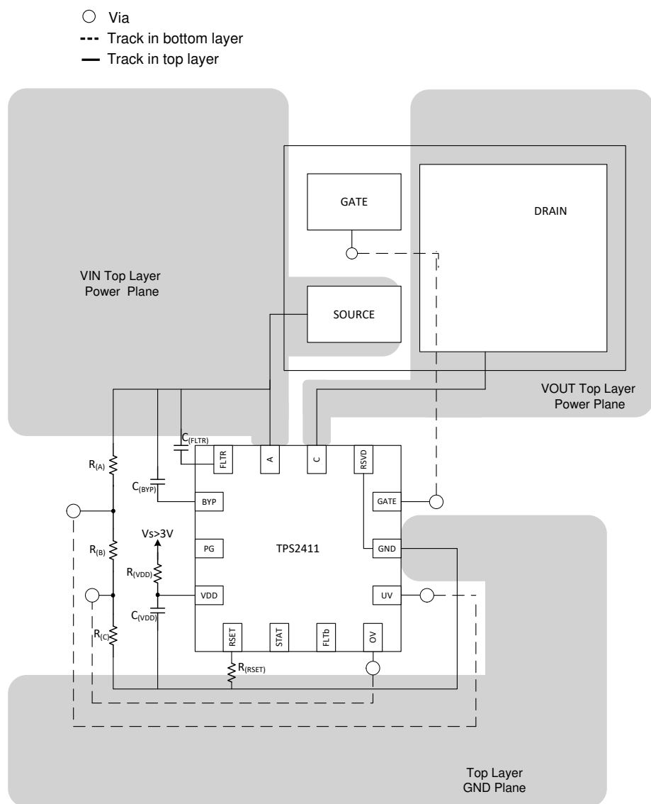
Figure 21. Example Layout
