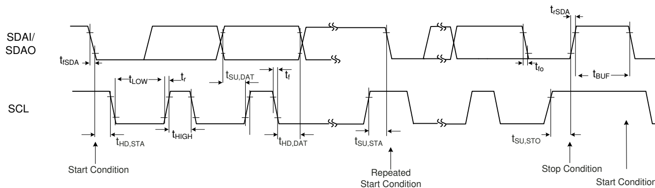
Figure 8-1. I²C Timings
