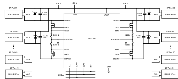
Simplified Schematic
