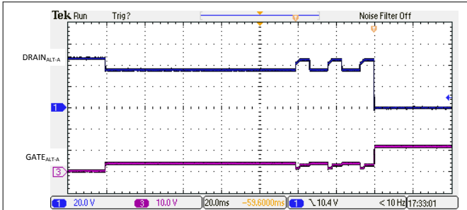
Figure 9-16. 2-Pair 3-Finger Classification and Turn-On
