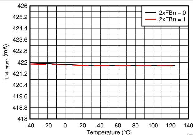
Figure 6-23. Inrush Current Limit vs Temperature
