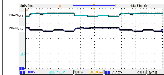
Figure 9-12. 4-Pair Low Resistance (11k \Omega ) Detection Signature
