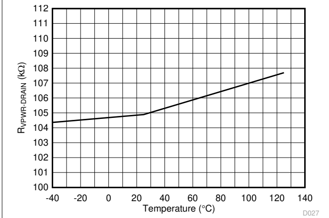
Figure 6-27. R_{\text{OFF}} (VPWR to DRAIN) vs Temperature
