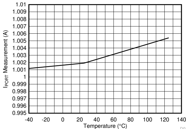
Figure 6-19. Port Current ADC Measurement (1 A) vs Temperature
