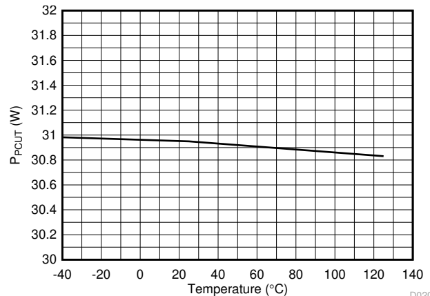
Figure 6-20. 2-Pair PCut Threshold (30W) vs Temperature
