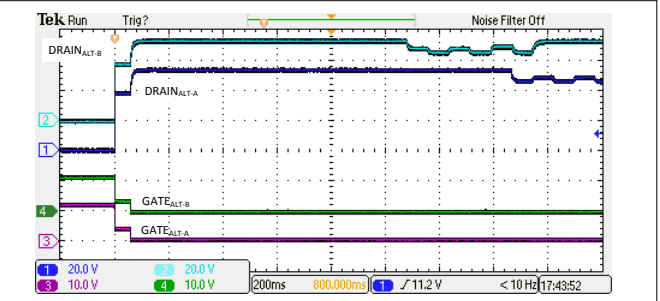
Figure 9-7. 4-Pair Backoff Due to I_{LIM} Fault
