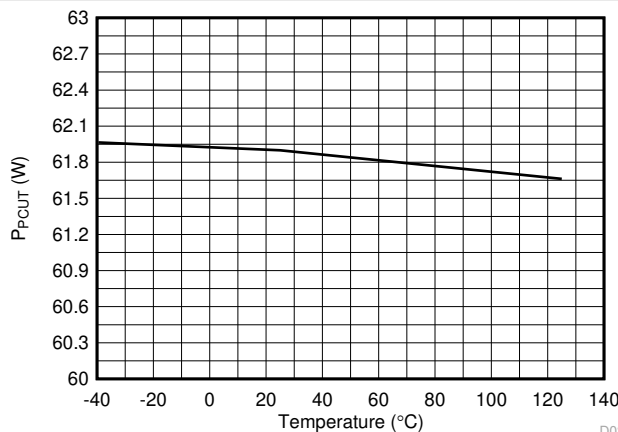
Figure 6-21. 4-Pair PCut Threshold (60W) vs Temperature
