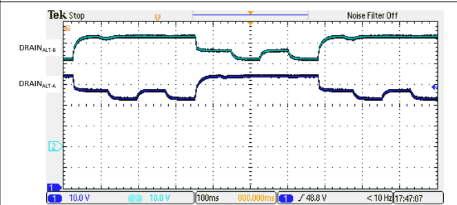
Figure 9-13. 4-Pair High Resistance (36k \Omega ) Detection Signature
