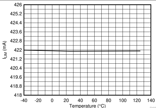
Figure 6-24. 1x Mode (2xFBn = 0) Current Limit vs Temperature
