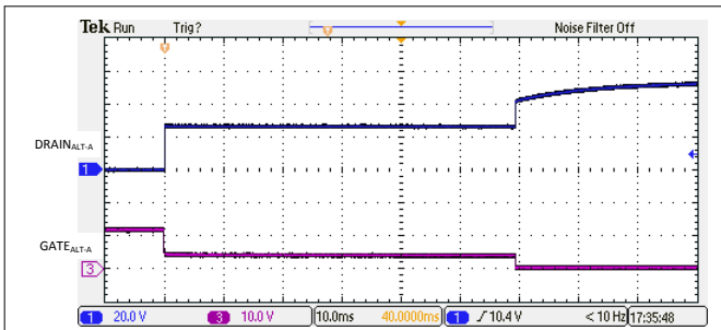
Figure 9-4. 2-Pair I_{LIM} Foldback and Turn-Off
