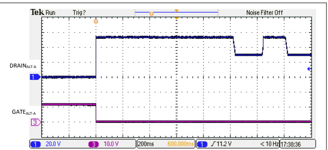
Figure 9-5. 2-Pair Backoff Due to PCut Fault
