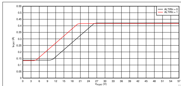
Figure 8-2. Foldback During Inrush (at Port Turn-On): I_{LIM} vs V_{port}
