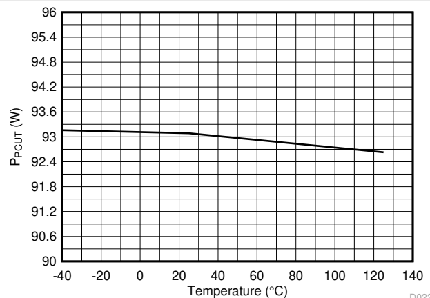
Figure 6-22. 4-Pair PCut Threshold (90W) vs Temperature
