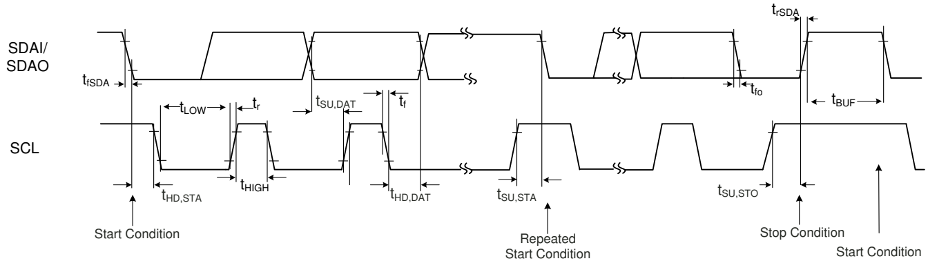
Figure 7-1. I 2 C Timings
