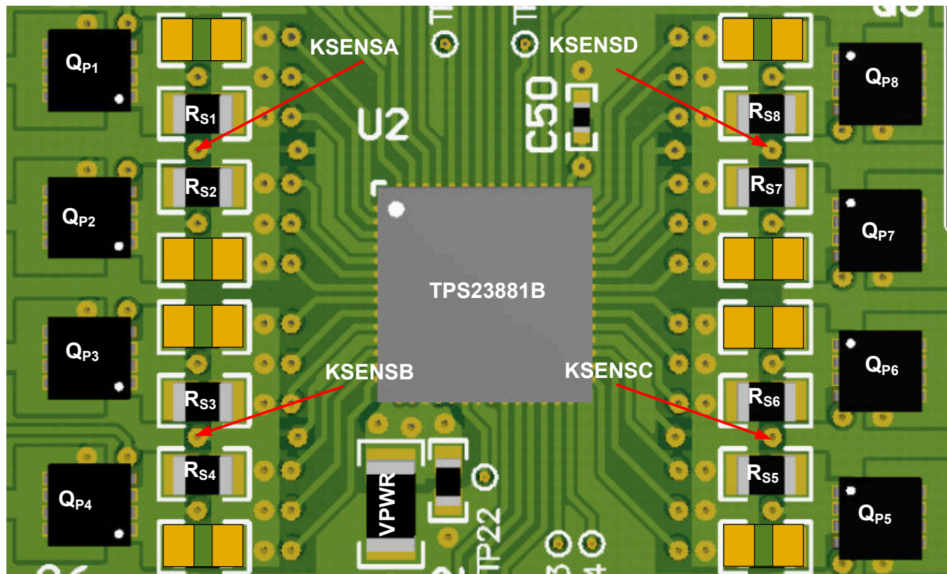
Figure 9-30. Eight Port Layout Example (Top Side)
