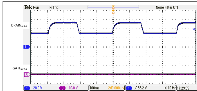
Figure 9-10. 2-Pair Open Circuit Detection Signature
