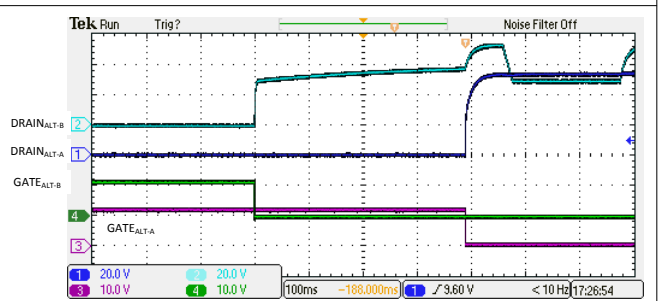
Figure 9-9. 4-Pair Single Signature Class 0-4 Disconnect
