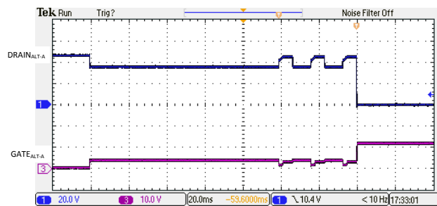
Figure 10-16. 2-Pair 3-Finger Classification and Turn-On
