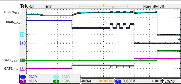
Figure 10-21. 4-Pair Single Signature 4-Finger Classification and Turn On
