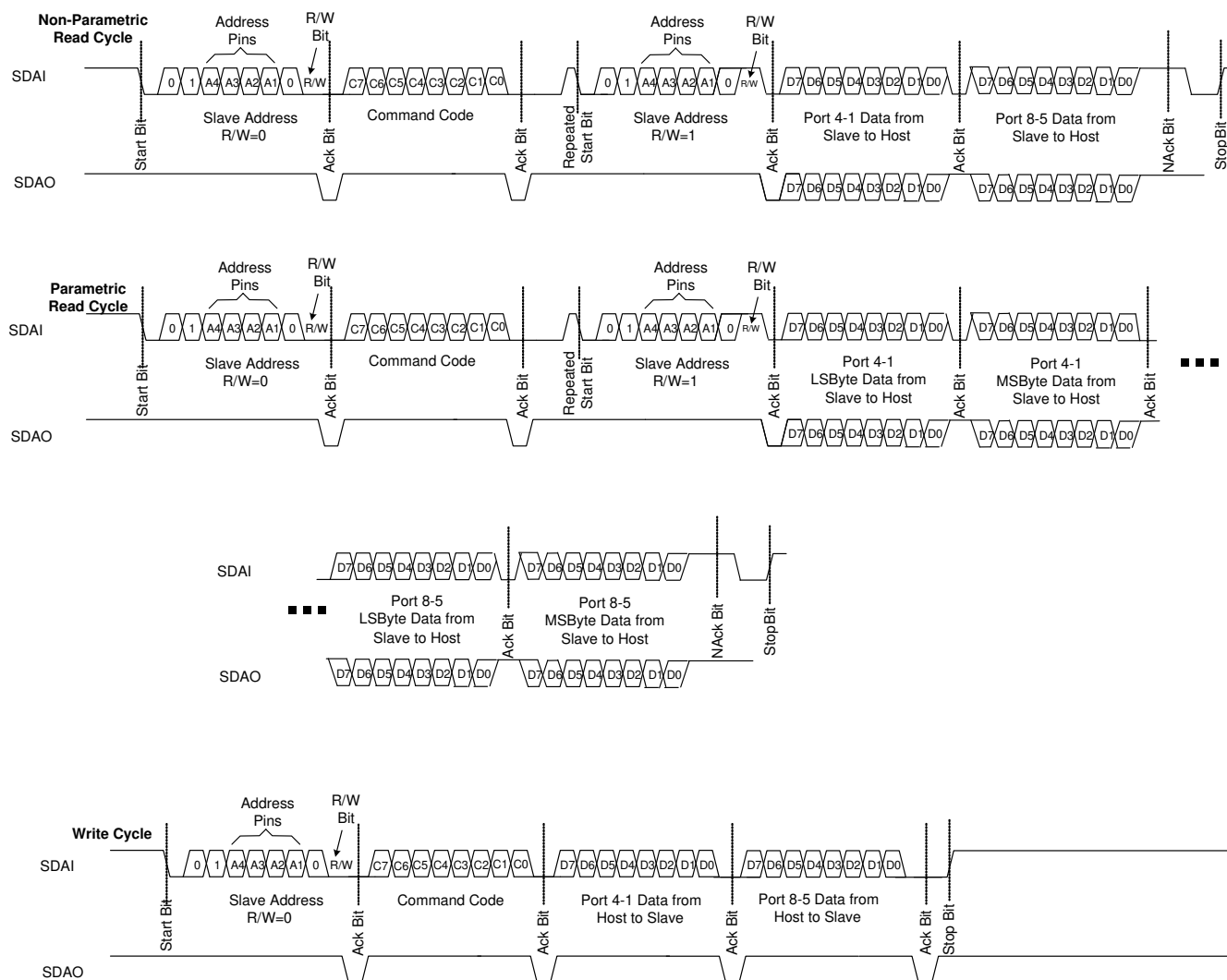
Figure 9-7. I 2 C interface Read and Write Protocol – Configuration B
