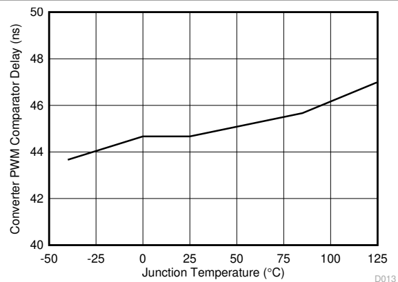
Figure 6-16. Converter PWM Comparator Delay vs Temperature
