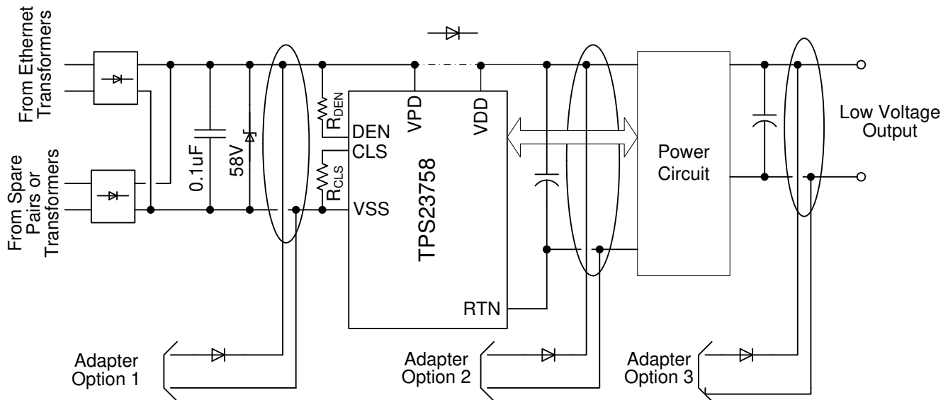
Figure 7-10. ORing Configurations
