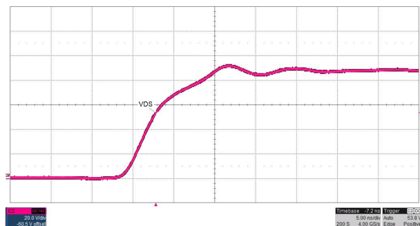
Figure 8-7. Slew Rate Adjust SRR = 0 \Omega
