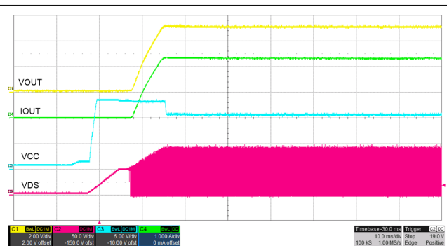
Figure 8-4. TPS23758 PSR Flyback Startup to Full Load
