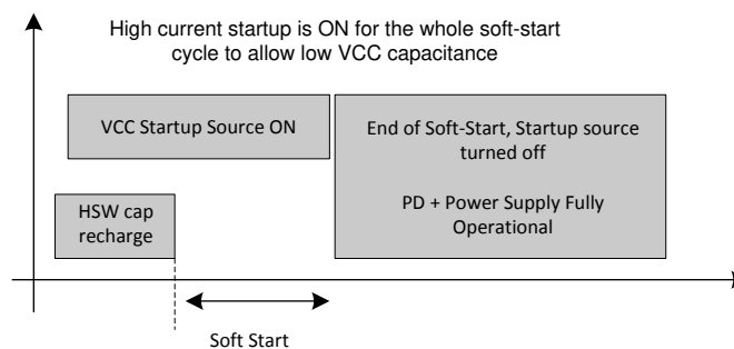
Figure 7-1. Advanced Startup
