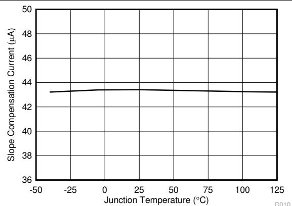
Figure 6-14. Current Slope Compensation Current vs Temperature
