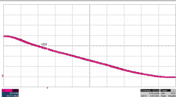
Figure 8-10. Slew Rate Adjust SRF = 100 \Omega
