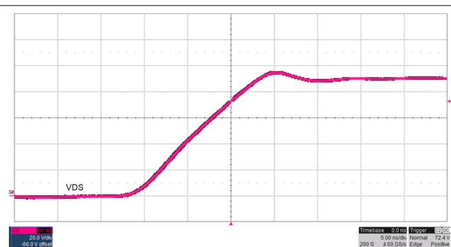
Figure 8-6. Slew Rate Adjust SRR = 10 Ω
