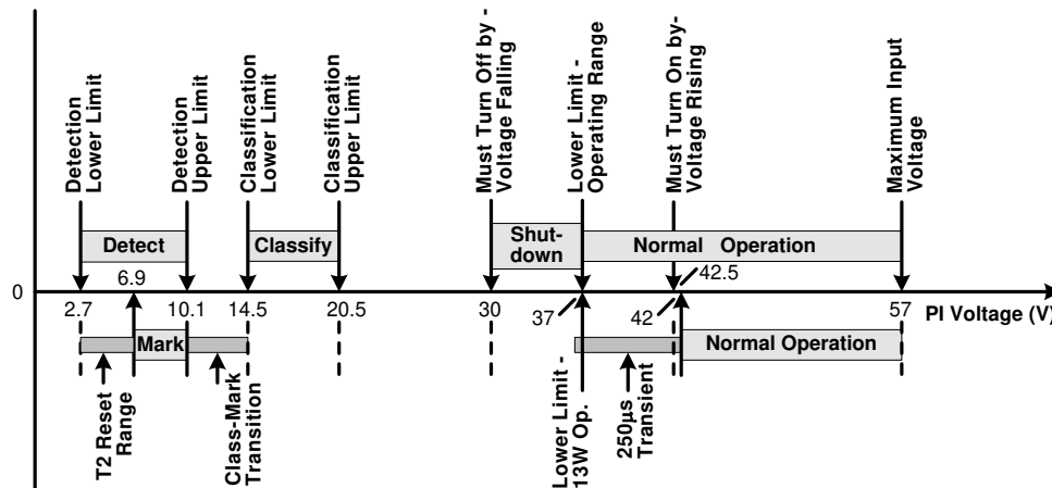
Figure 8-5. Operational States
