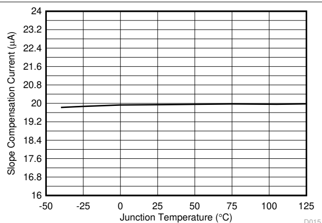
Figure 7-14. Current Slope Compensation Current vs Temperature
