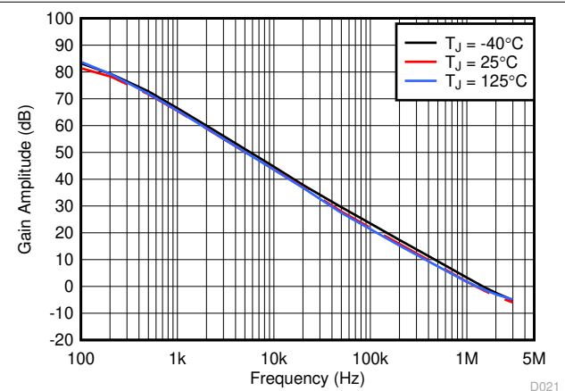
Figure 7-18. Error Amplifier Gain vs Frequency
