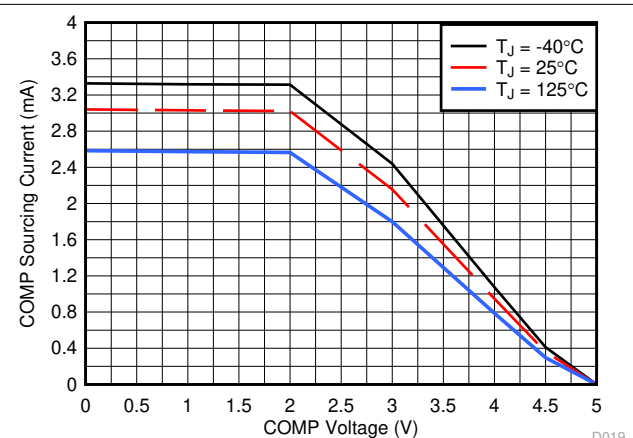
Figure 7-16. Error Amplifier Source Current
