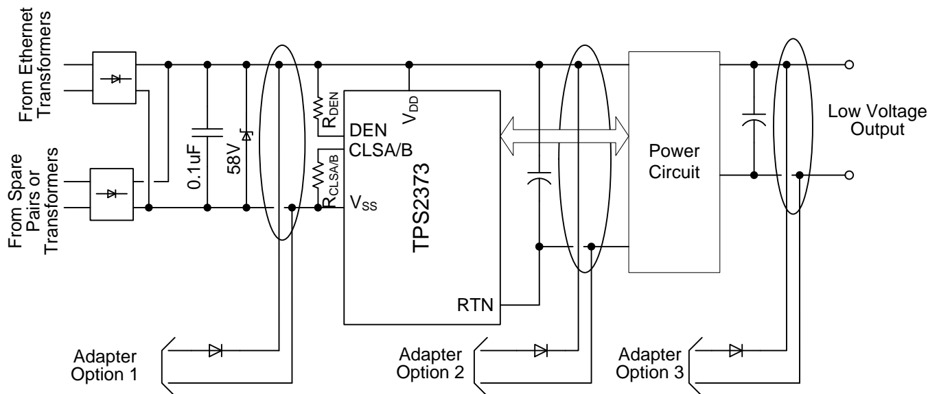
Figure 29. ORing Configurations
