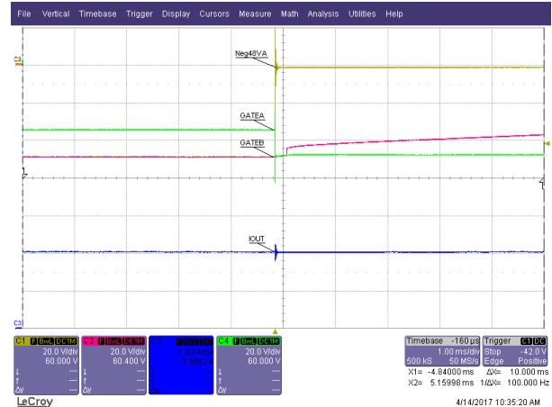
Figure 40. VinA Short
