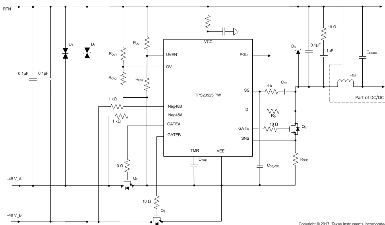
Figure 12. Application Diagram for Design Example
