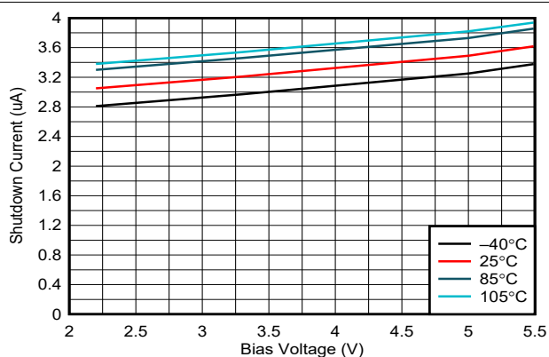
Figure 6-5. VBIAS Shutdown Current vs Bias Voltage
