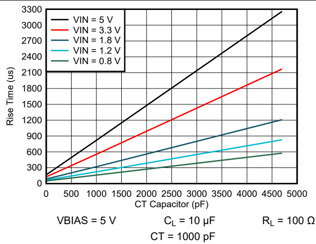
Figure 6-10. Rise Time vs CT Capacitor
