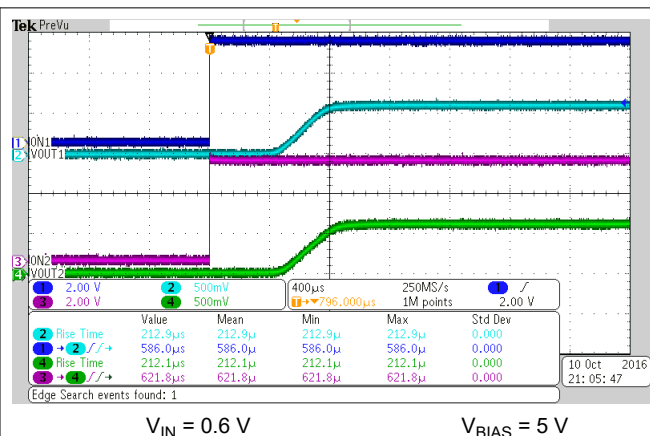
Figure 6-32. Turnon Response Time
