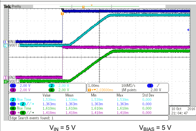
Figure 6-34. Turnon Response Time
