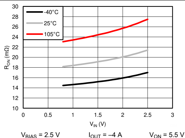
Figure 7-12. R_{ON} vs V_{IN}
