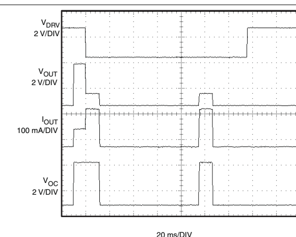
Figure 21. t_{RESTART} Response
