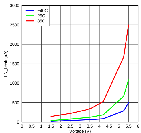
Figure 4. Input Current, Leak vs Input Voltage
