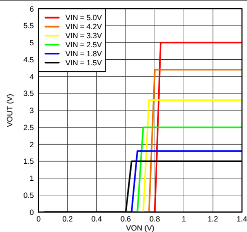
Figure 2. On Input Threshold
