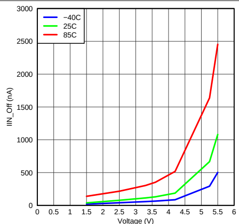
Figure 6. Input Current, Off vs Input Voltage
