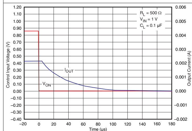
Figure 26. t_{OFF} Response
