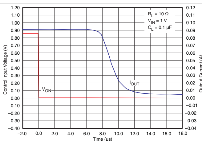
Figure 27. t_{OFF} Response
