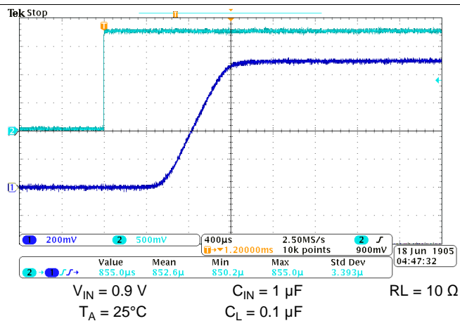
Figure 16. Turn-On Response
