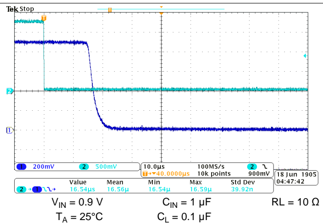
Figure 17. Turn-Off Response
