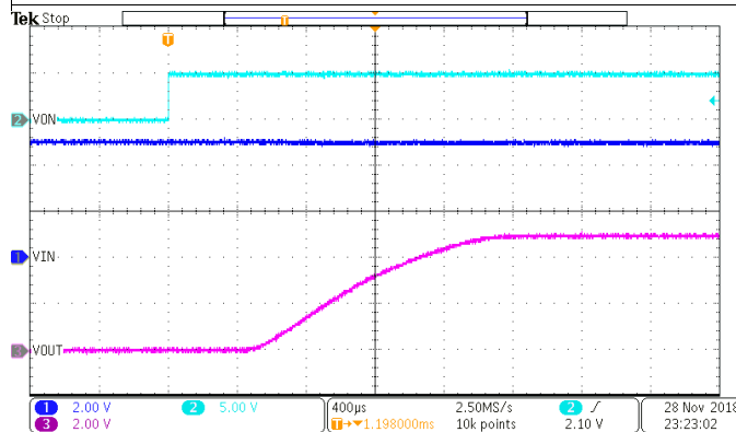
Figure 18. Rise Time with VIN = 1.8 V
