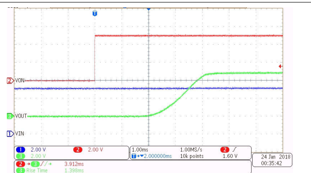
Figure 7-14. Turn-On at 5 V (CT = 1000 pF)
