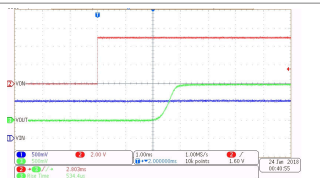
Figure 7-18. Turn-On at 1 V (CT = 1000 pF)
