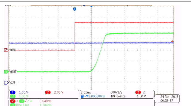
Figure 7-16. Turn-On at 3.6 V (CT = 1000 pF)
