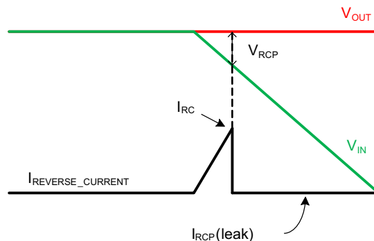
Figure 49. Reverse Current
