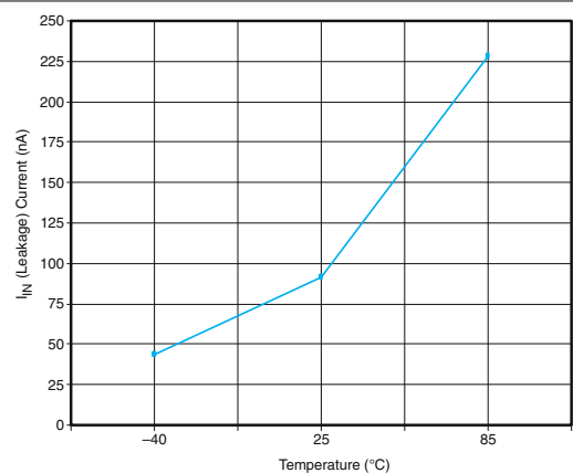
Figure 7-9. I_{IN(Leakage)} vs Temperature ( V_{IN} = 3.3\text{ V} )
