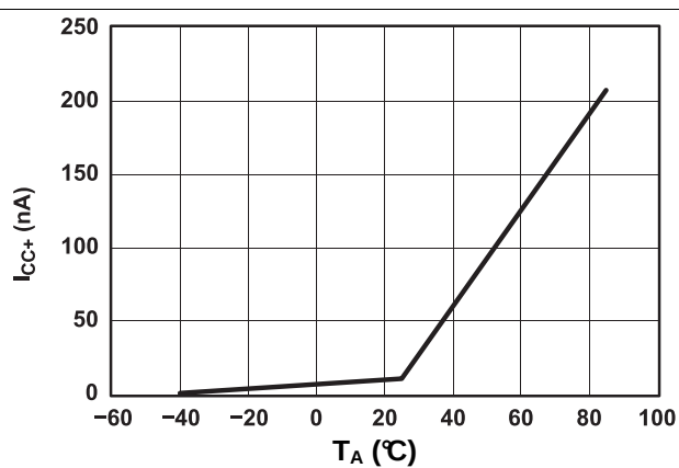
Figure 7. Power-Supply Current vs Temperature ( V_{BIAS} = 5 V)
