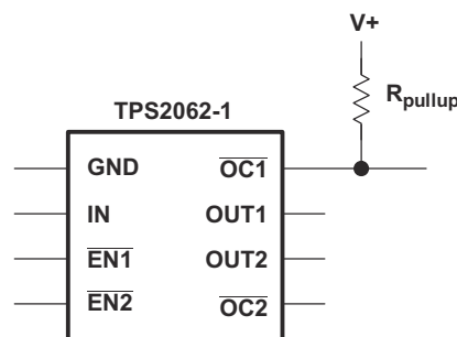
Figure 8-2. Typical Circuit for the \overline{OC} Pin
