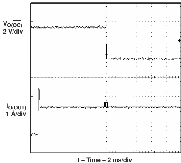
Figure 6-8. 2- \Omega Load Connected to Enabled Device
