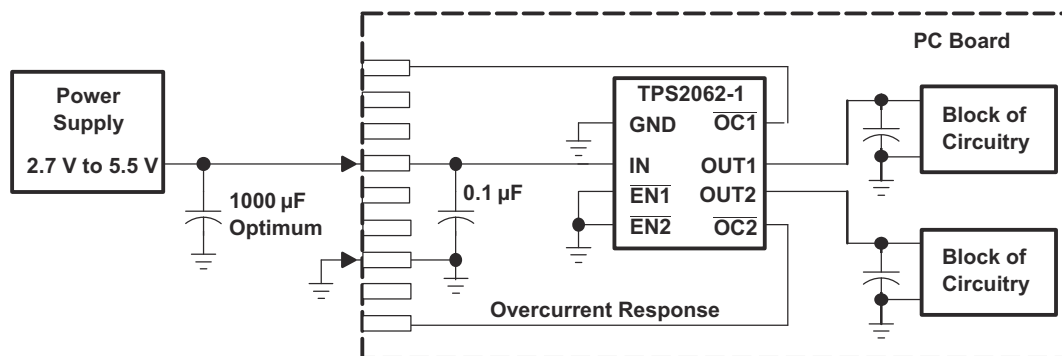
Figure 8-6. Typical Hot-Plug Implementation
