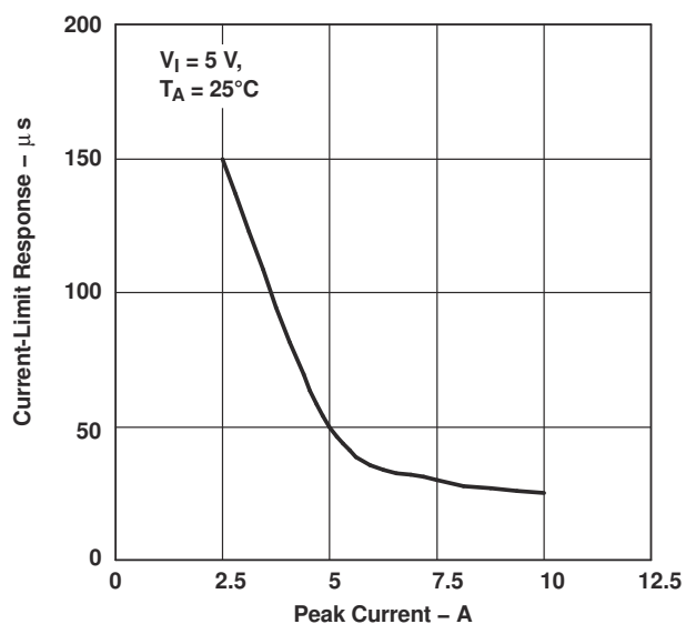
Figure 5-13. CURRENT-LIMIT RESPONSE vs PEAK CURRENT
