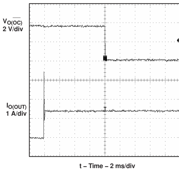
Figure 6-9. 1- \Omega Load Connected to Enabled Device
