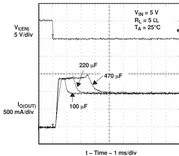
Figure 6-7. Inrush Current With Different Load Capacitance
