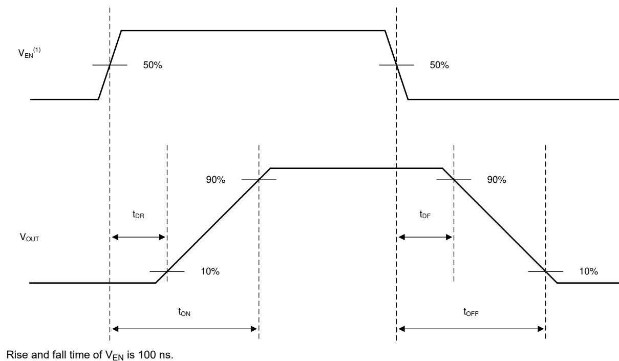
Figure 6-2. Switching Characteristics Definitions
