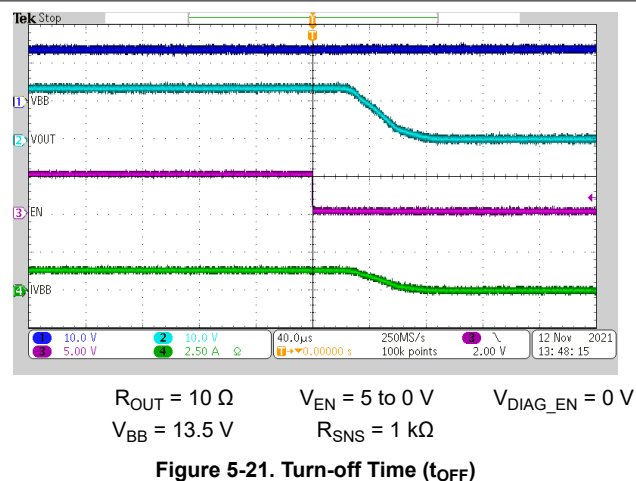
Figure 5-21. Turn-off Time ( t_{OFF} )
