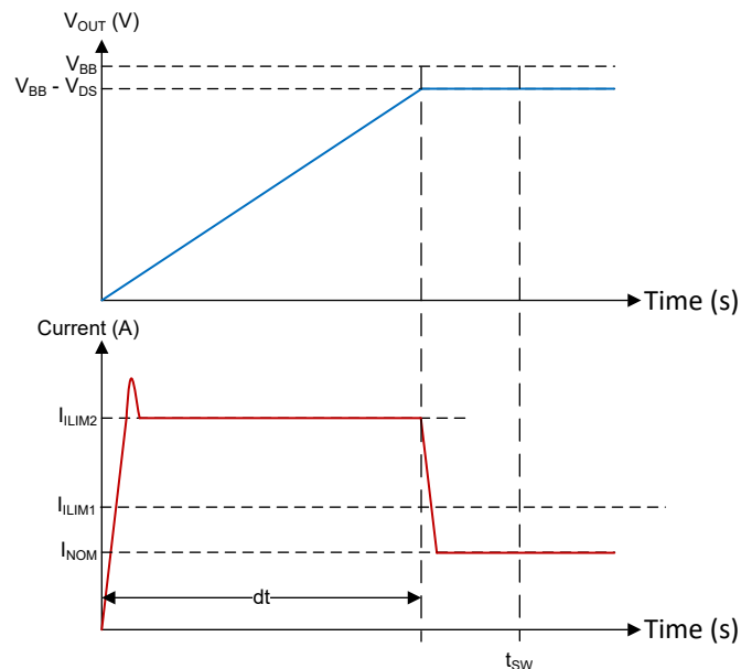
Figure 8-3. Capacitive Charging Changing Current Limit
