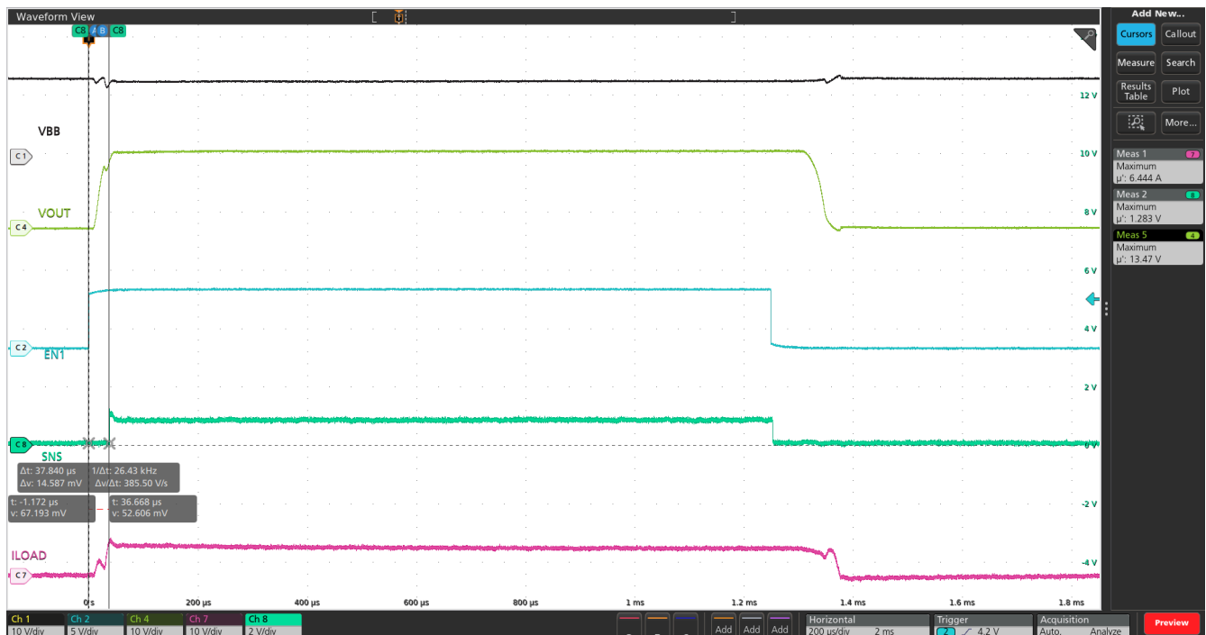
Figure 8-6. SNS Response Time with EN ( t_{SNS10N3} )
