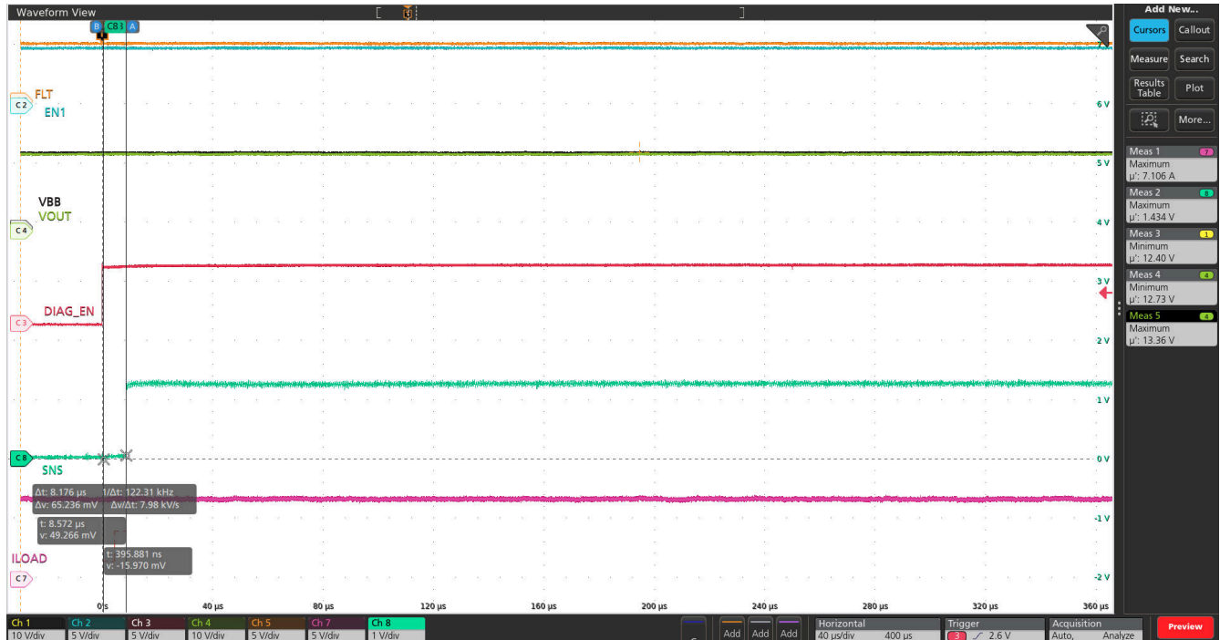
Figure 8-5. SNS Response Time with DIAG_EN ( t_{SNS10N1} )
