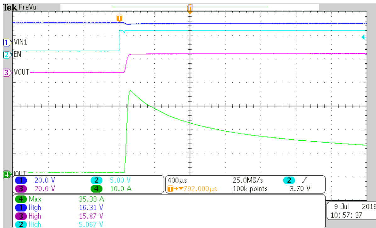
Figure 10-5. TPS1HB35-Q1 Version F 21W Bulb Inrush
