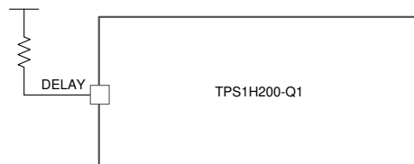
Figure 7-6. Auto-Retry-Mode Connection
