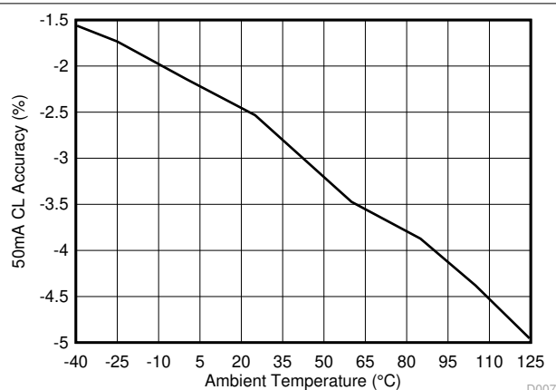
Figure 5-9. Current-Limit Accuracy at 50 mA
