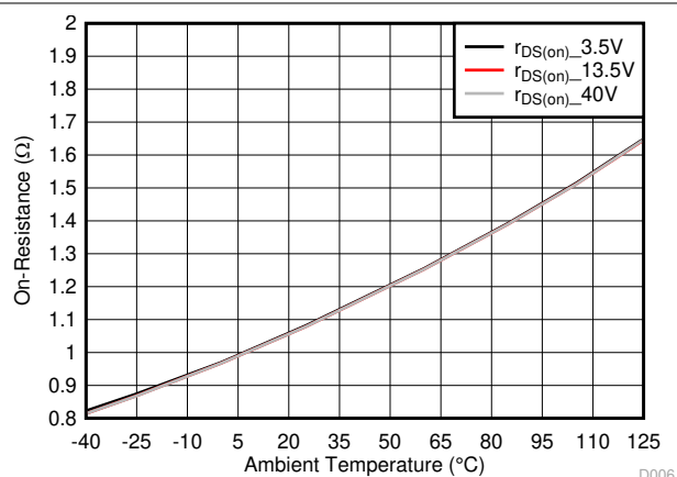
Figure 5-8. FET On-Resistance
