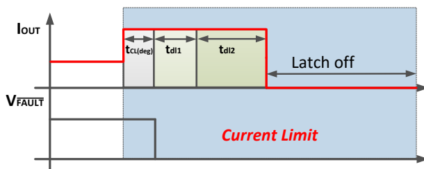
Figure 6-5. Latch-Off-Mode Example
