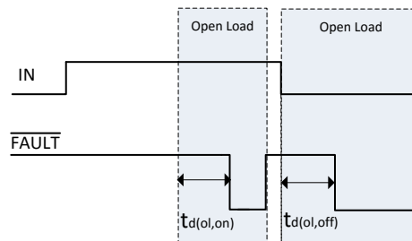
Figure 5-2. Open-Load Blanking-Time Characteristic
