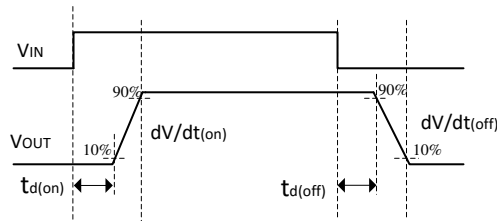
Figure 5-1. Output Delay Characteristics
