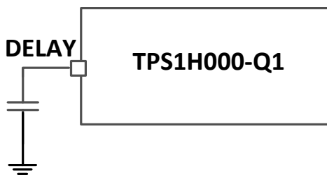
Figure 6-4. Latch-Off-Mode Connection
