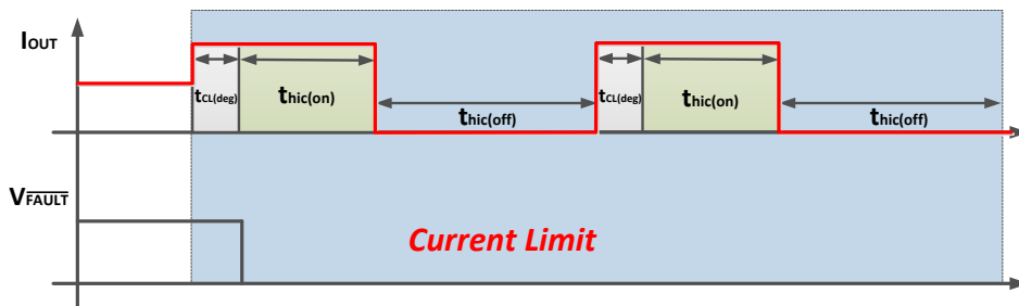
Figure 6-7. Auto-Retry-Mode Example
