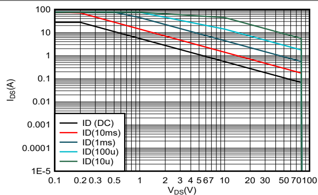
Figure 6-14. Allowed Operating Area (AOA) in Steady State
