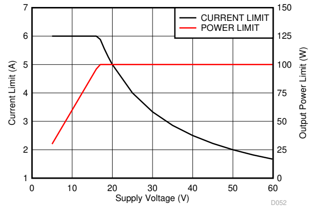
TPS16632 R_{(PLIM)} = 100\text{ k}\Omega R_{(ILIM)} = 3\text{ k}\Omega
