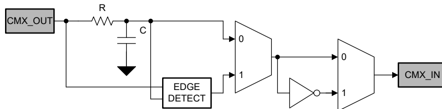
Figure 7-24. Deglitch Filter or Edge Detector Block Diagram
