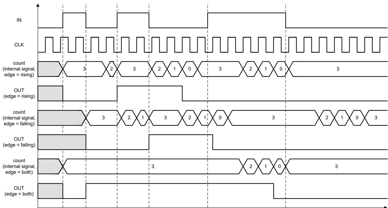
Figure 7-19. Frequency comparator output timing example (DATA = 3)
