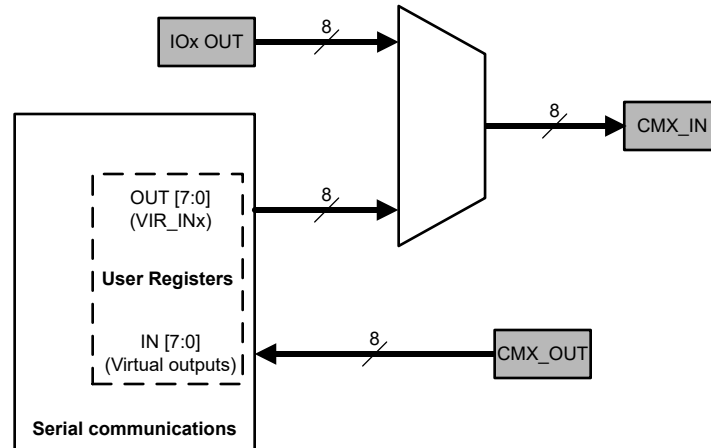
Figure 7-60. Serial Communications Block Diagram
