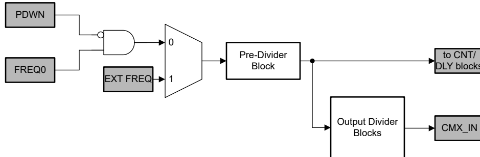
Figure 7-48. Fixed frequency oscillator block diagram
