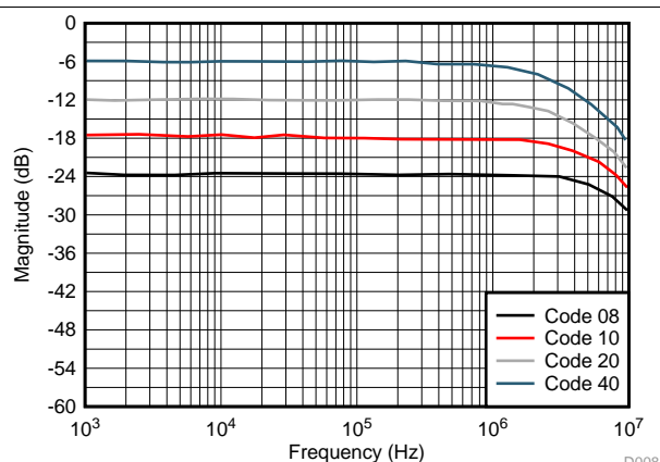
Figure 8. Frequency Response
