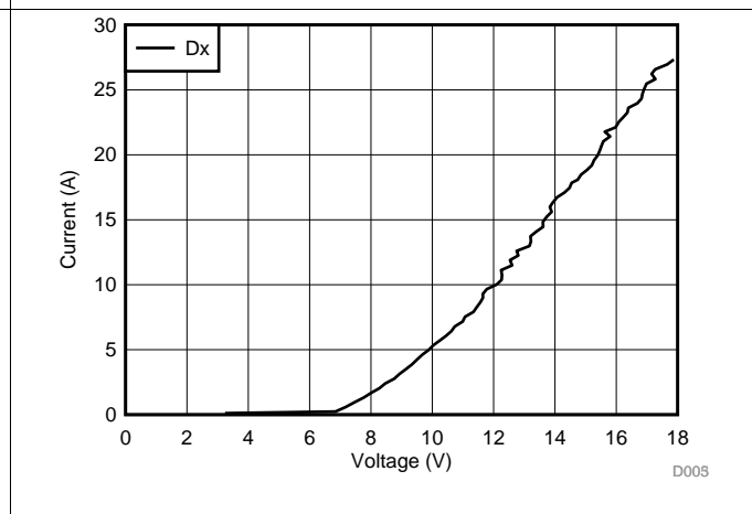
Figure 28. Dx TLP Curve
