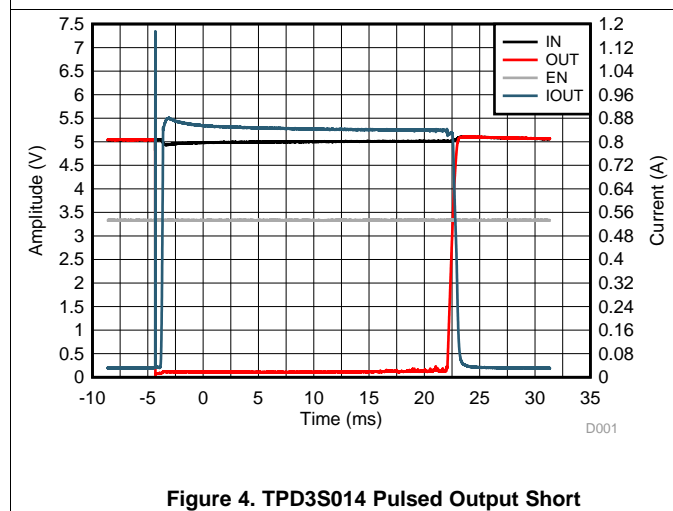
Figure 4. TPD3S014 Pulsed Output Short
