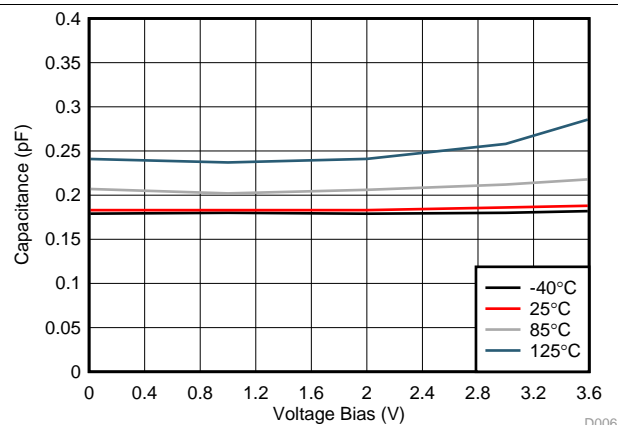
Figure 6. Capacitance vs. Bias Voltage (DPL Package)
